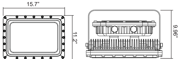
D2L140 (Dominus 2) Dimension Diagram (100W / 120W / 150W / 200W)
