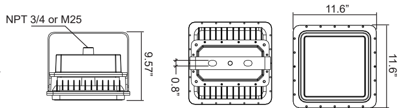
D1L140 (Dominus 1) Dimension Diagram (20W / 60W / 80W)
